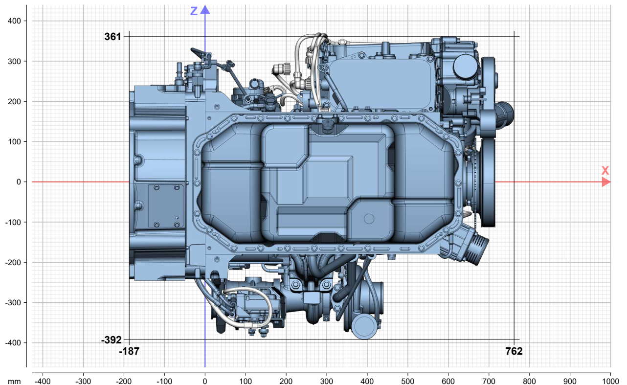
Bottom view
