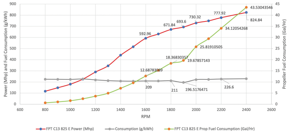
FPT C13 825 E Performance
