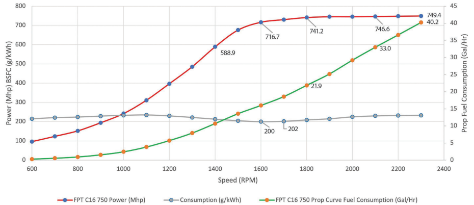
FPT C16 750@2300 Performance Curve
